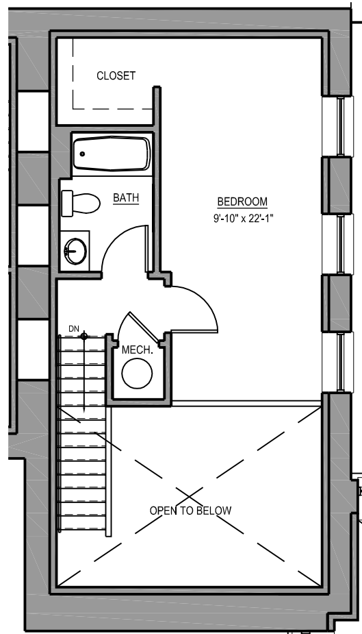
1 BEDROOM TOWNHOUSE : +/- 603 SF (UPPER) UNIT 1124
